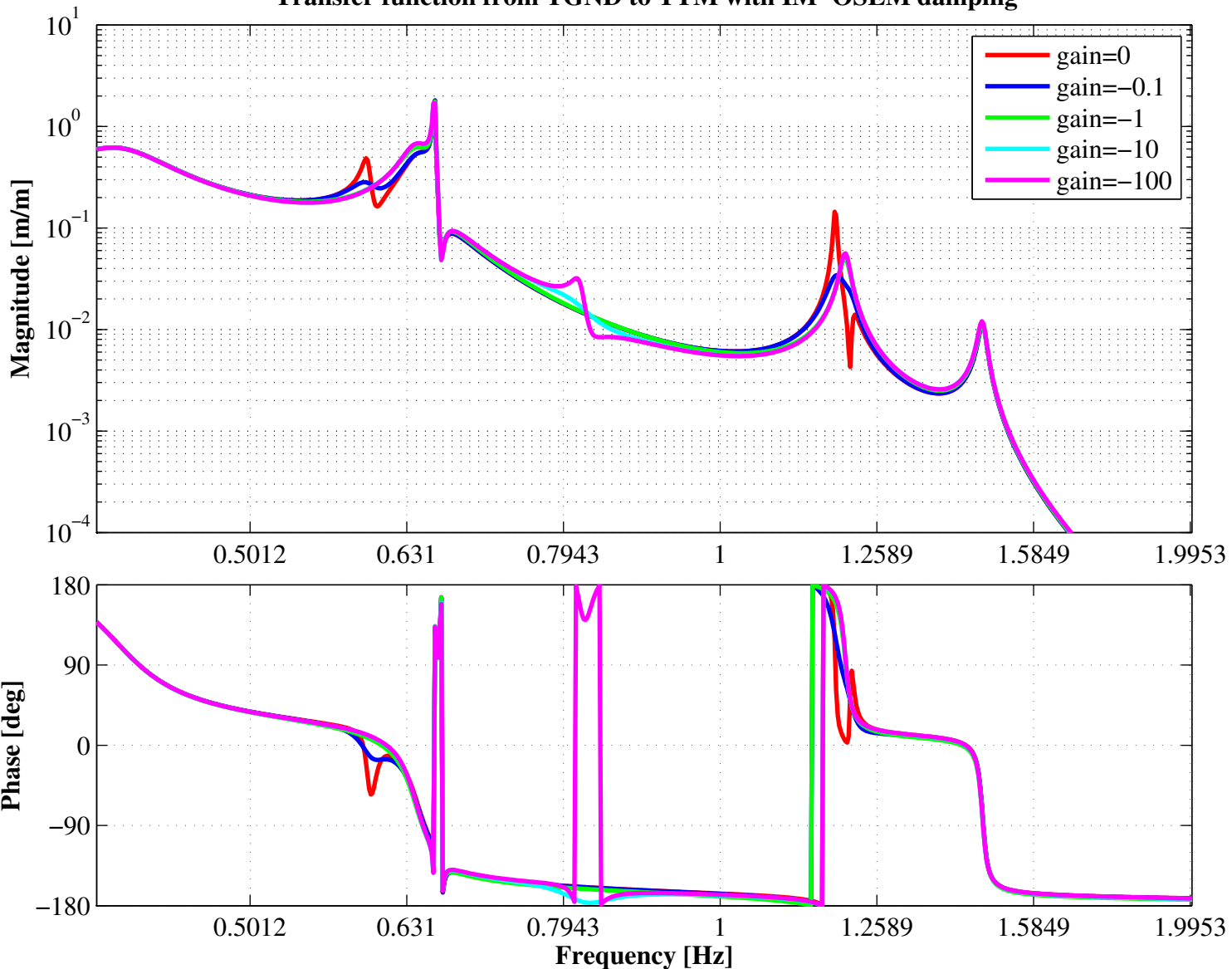
Transfer function from TGND to TTM with IM-OSEM damping
