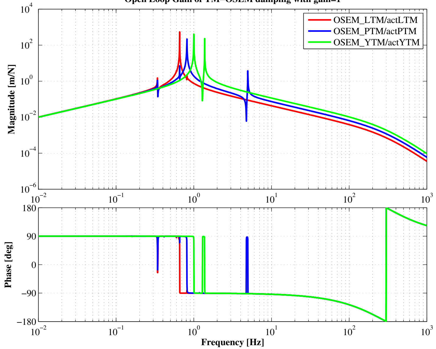
Open Loop Gain of TM-OSEM damping with gain=1
