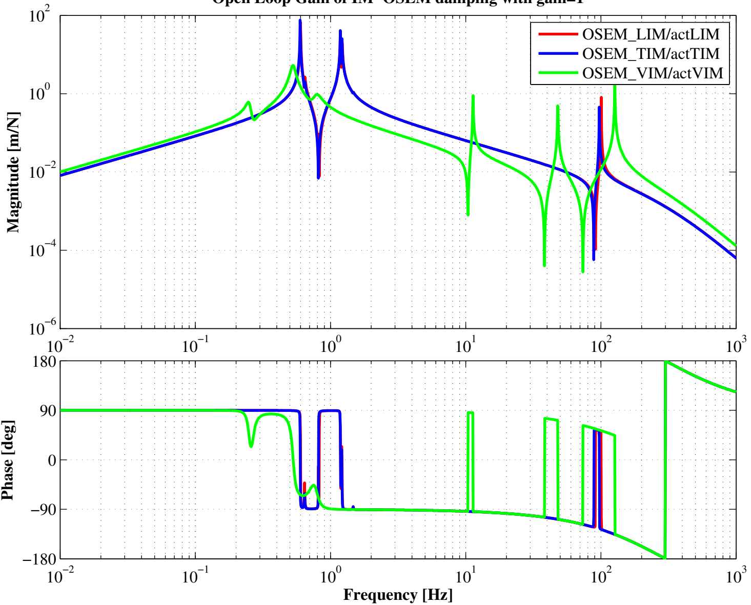
Open Loop Gain of IM-OSEM damping with gain=1
