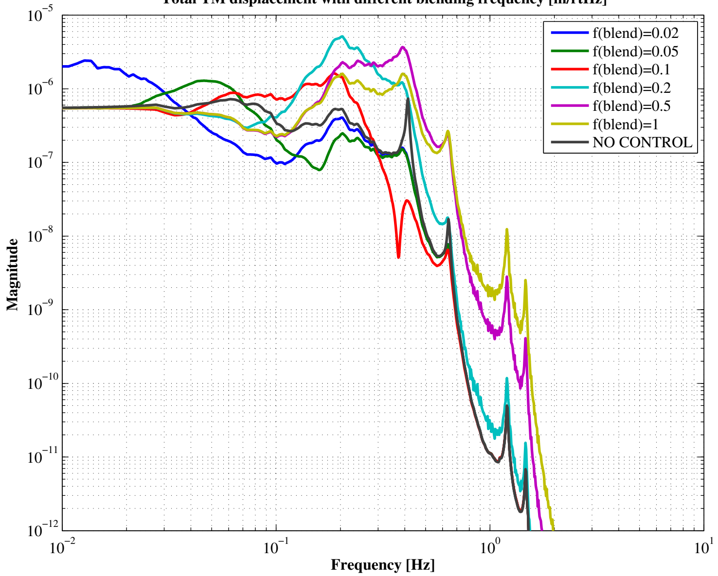
Total TM displacement with different blending frequency [m/rtHz]
