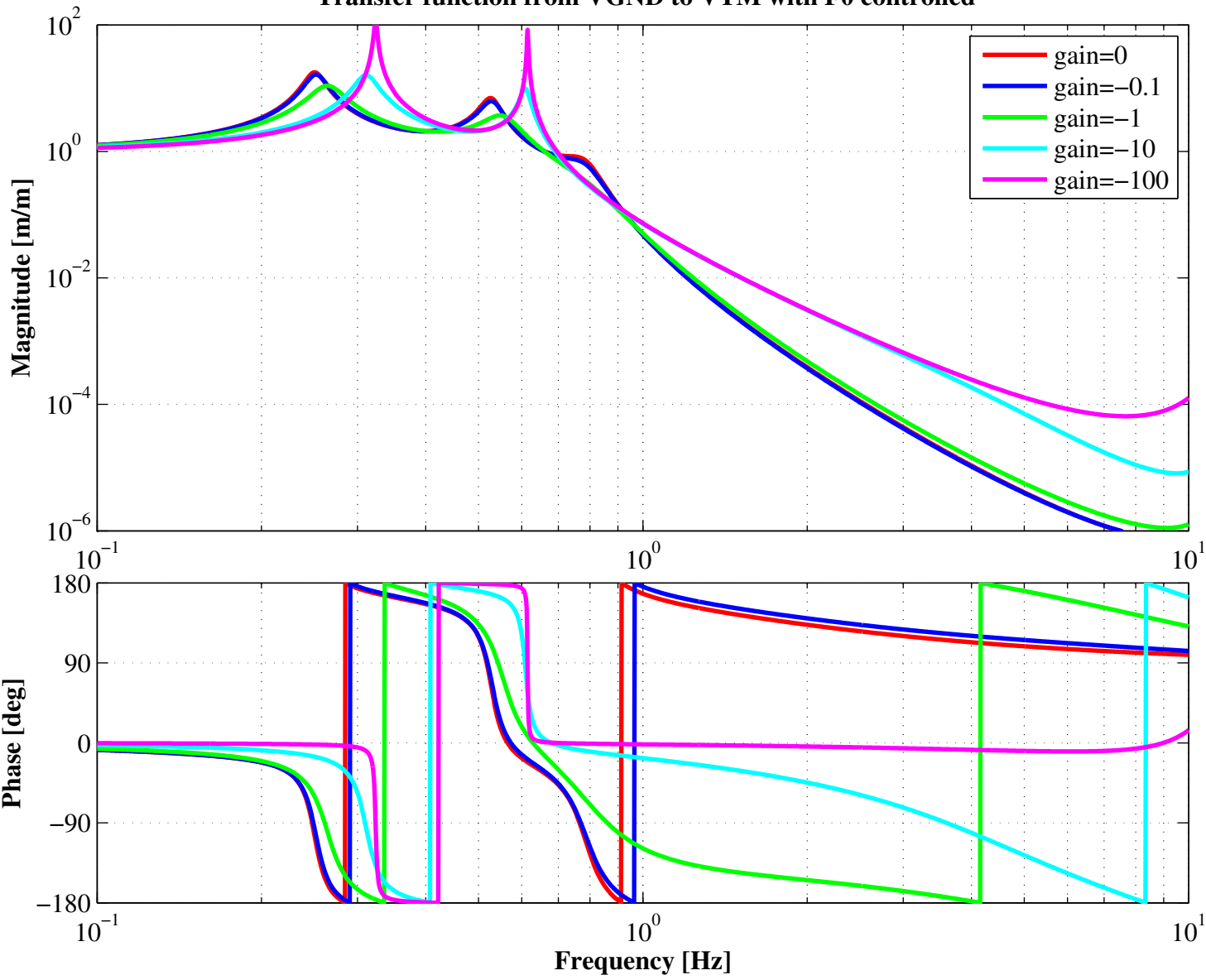
Transfer function from VGND to VTM with F0 controlled
