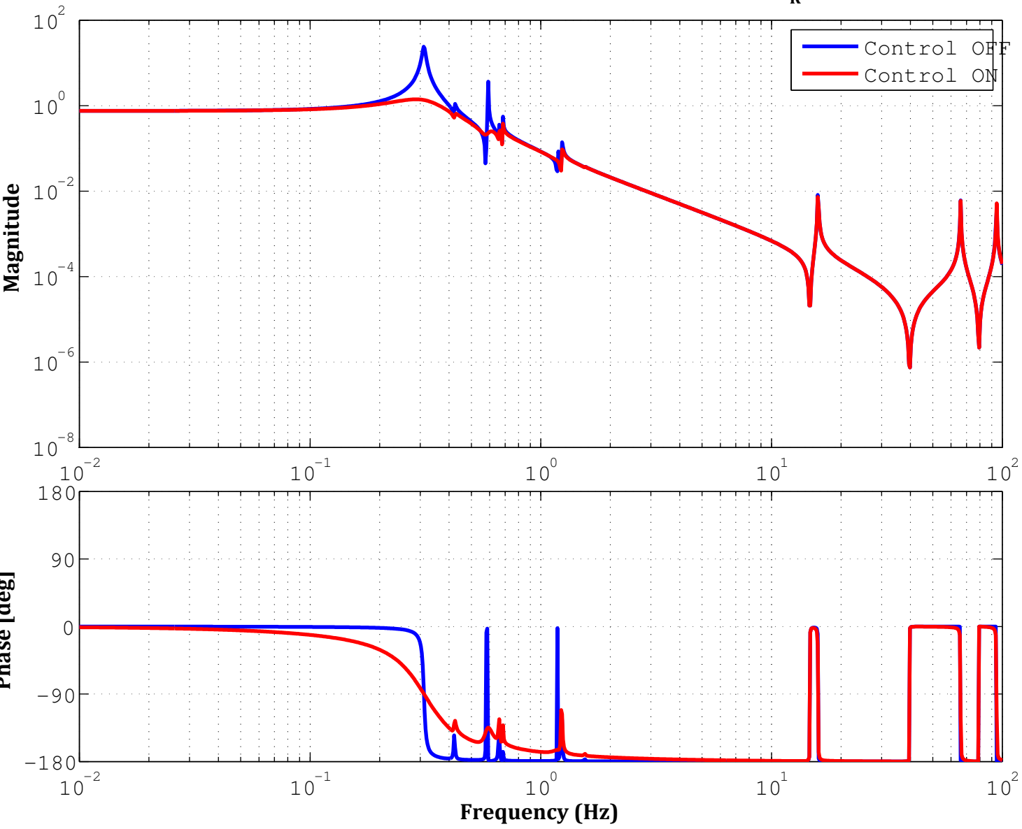
Transfer Function Bode Plot from actRIM to OSEM IM
