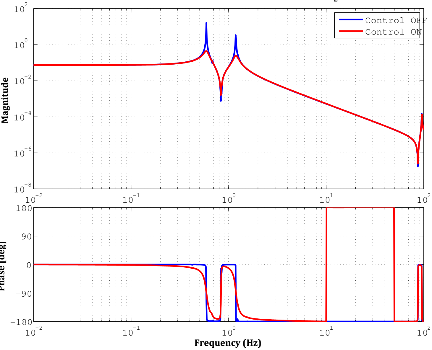
Transfer Function Bode Plot from actLIM to OSEM IM
