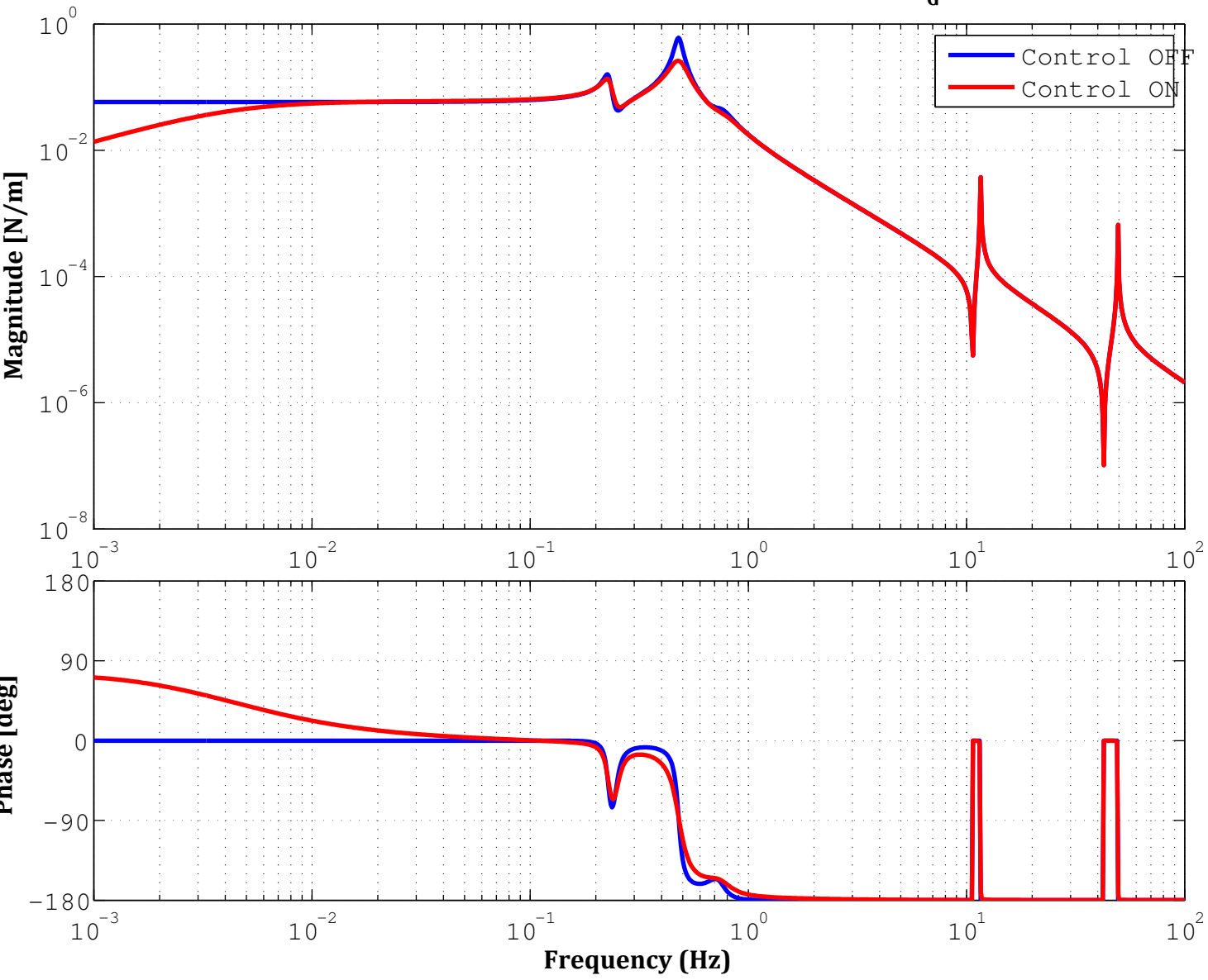
Transfer Function Bode Plot from actGASBF to LVDT G^{ASBF}
