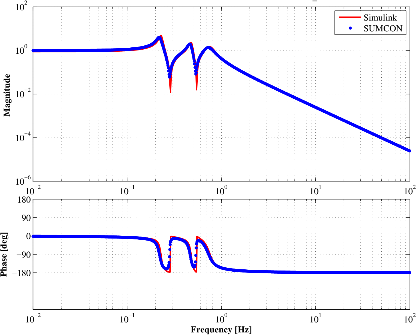
Transfer Function Bode Plot from actGASF0 to LVDT_GASF0
