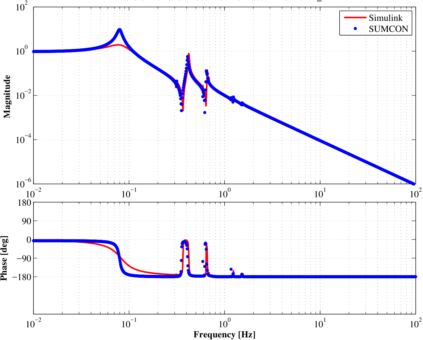
Transfer Function Bode Plot from actTIP to LVDT_TIP
