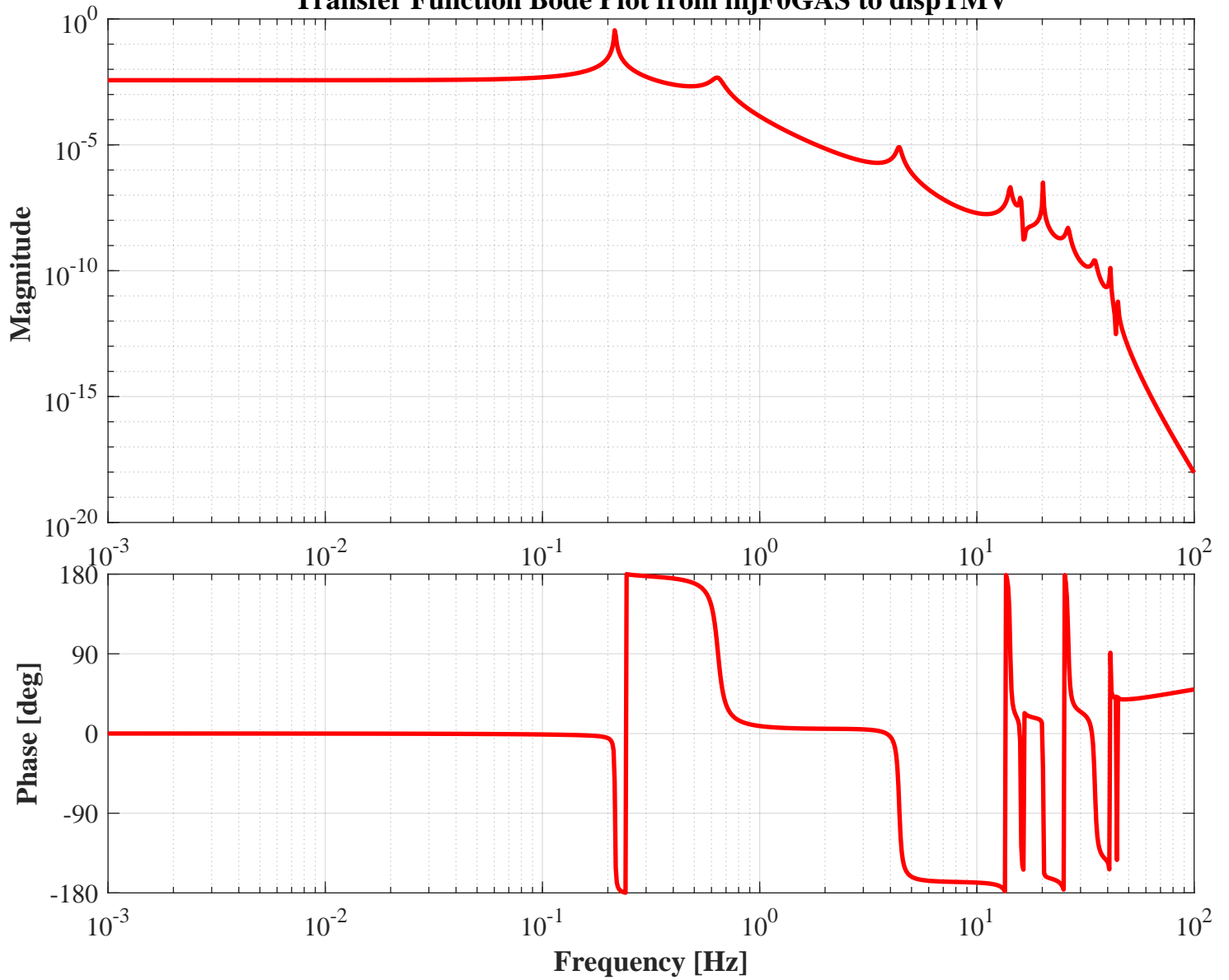
Transfer Function Bode Plot from injF0GAS to dispTMV
