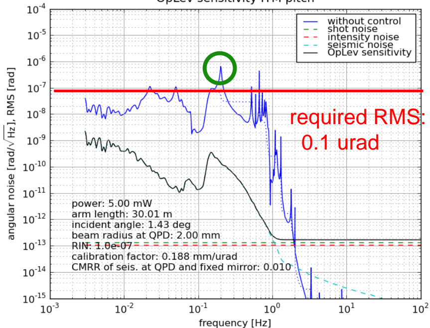
OpLev sensitivity ITM pitch
