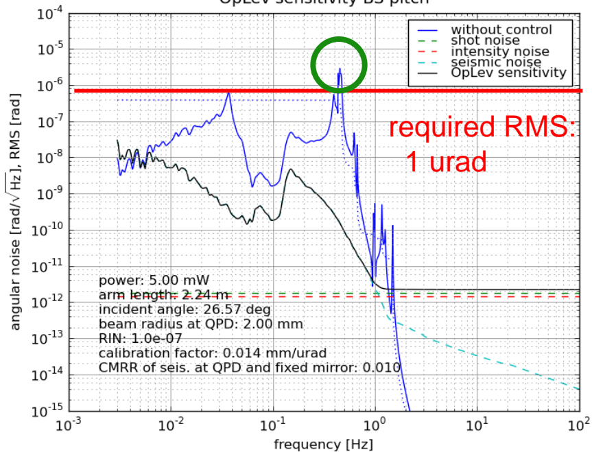
OpLev sensitivity BS pitch
